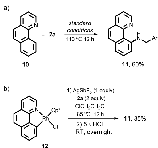
Scheme 7. a) Catalytic amination of benzo[ h ]quinoline ( 10 ). b) Stoichiometric reaction with the cyclometalated rhodium complex 12 . Ar = 3,5-(CF 3 ) 2 C 6 H 3 .
